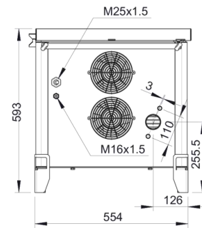
DIMENSION (SC6M-3)
