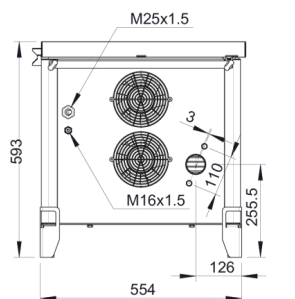
DIMENSION (SC6M-3)
