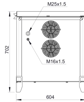
DIMENSION (SC6M-2)
