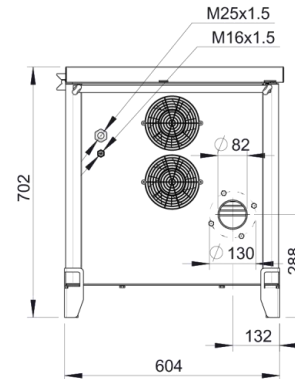
DIMENSION (SC8M-2)
